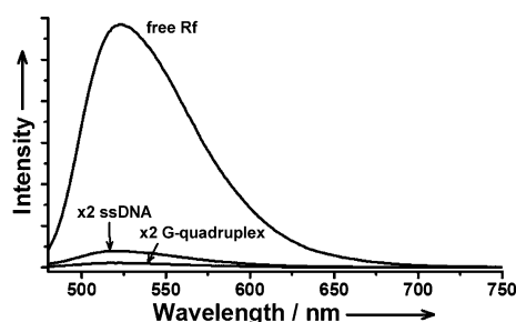
Figure 1. Fluorescence spectra of free Rf, single-stranded Rf-G-q and quadruplex Rf-G-q in 10 mM Tris-HCl buffer (pH 7.4) at room temperature ( \lambda_{ex} = 450 nm).
